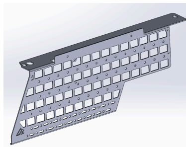
Passenger Upper Panel (1):
